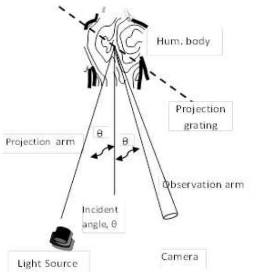
Fig. 2. Setup for projection moiré
